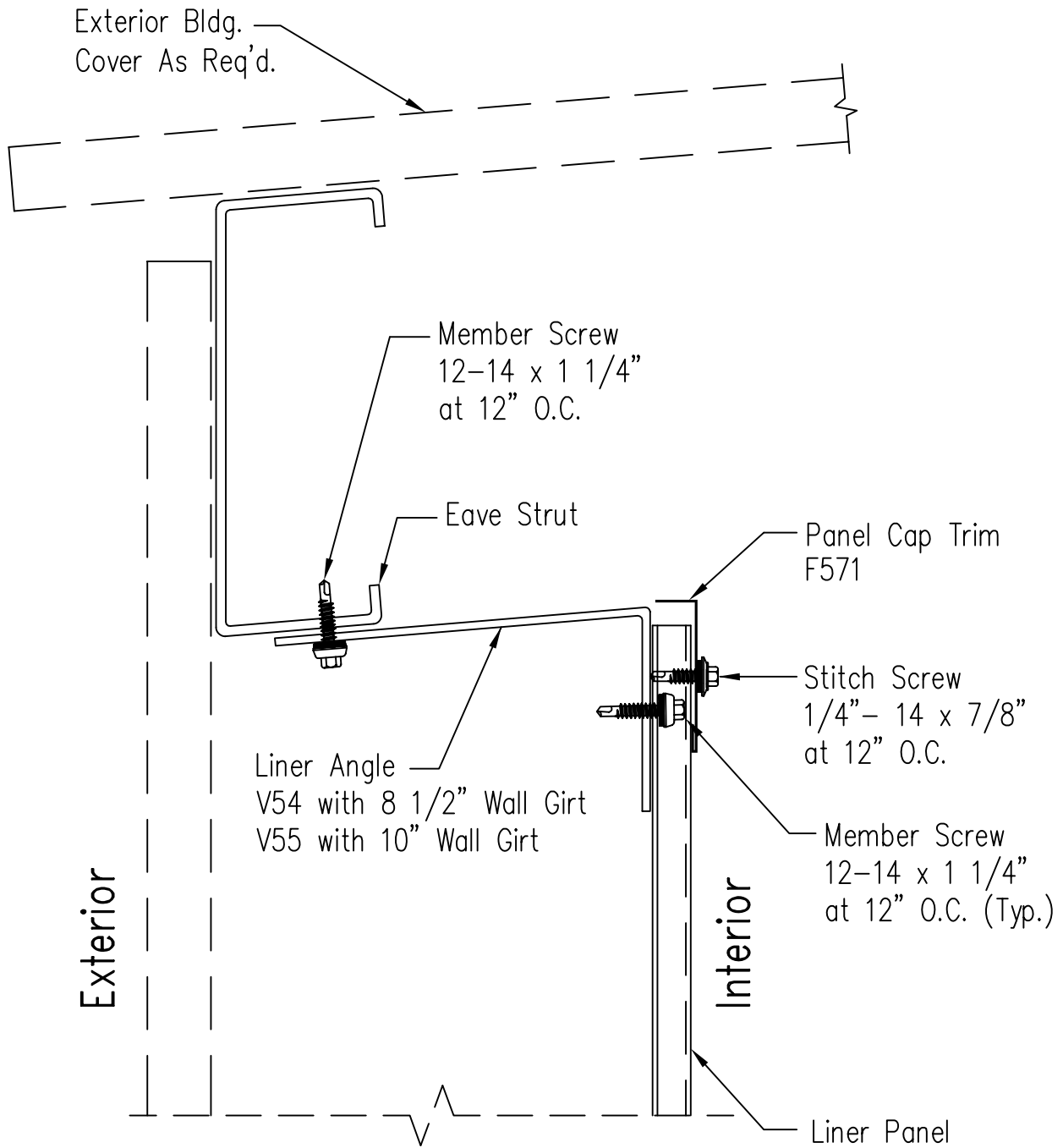
Section At Eave
