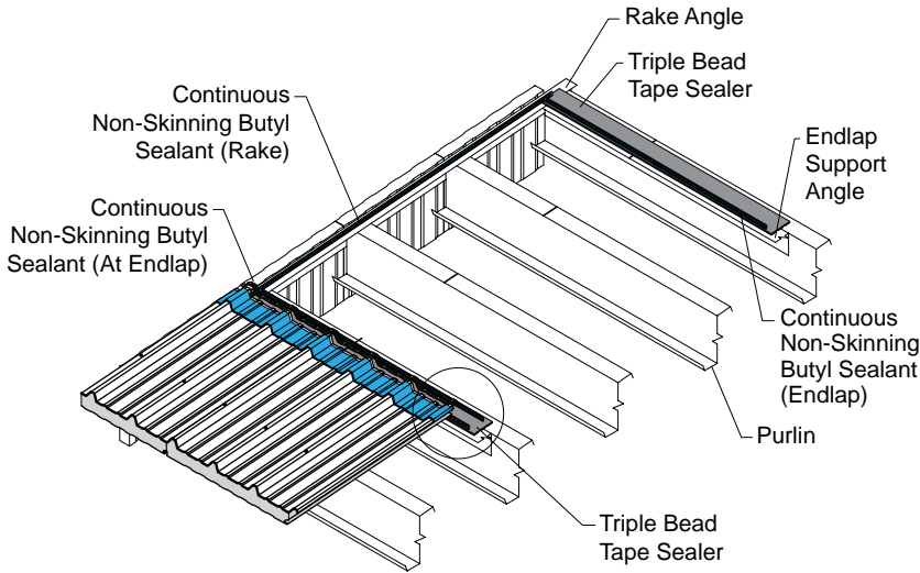
Endlap Panel Sealant
