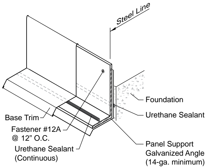
Base Assembly Without Sheeting Notch
