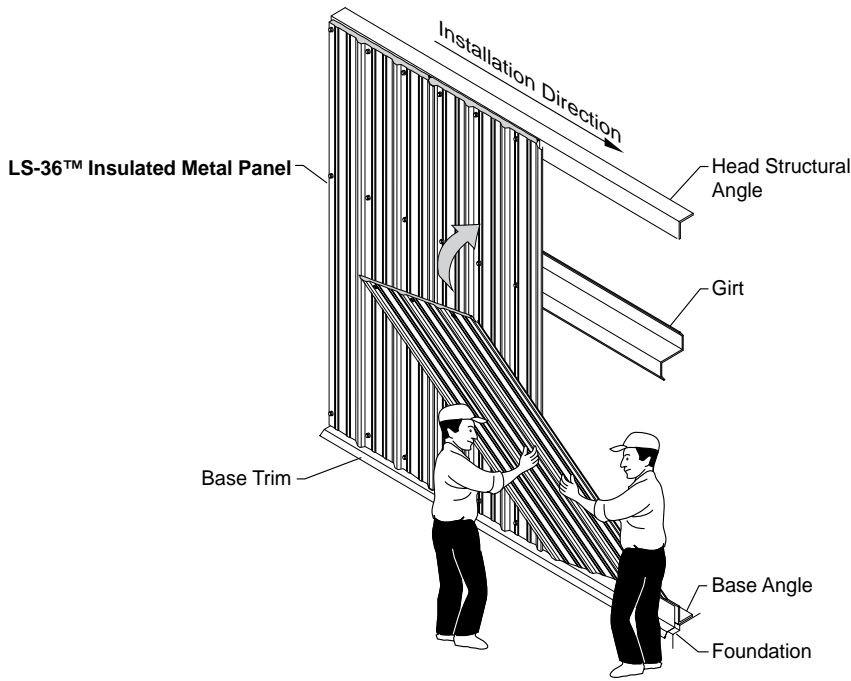
Manual Panel Setting
