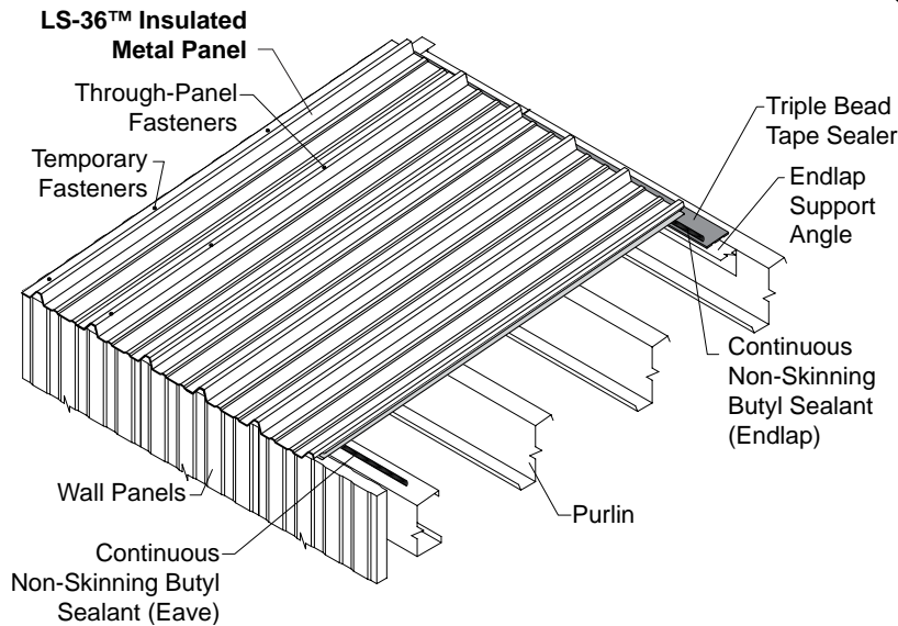
Subsequent Runs Eave Panel Installed
