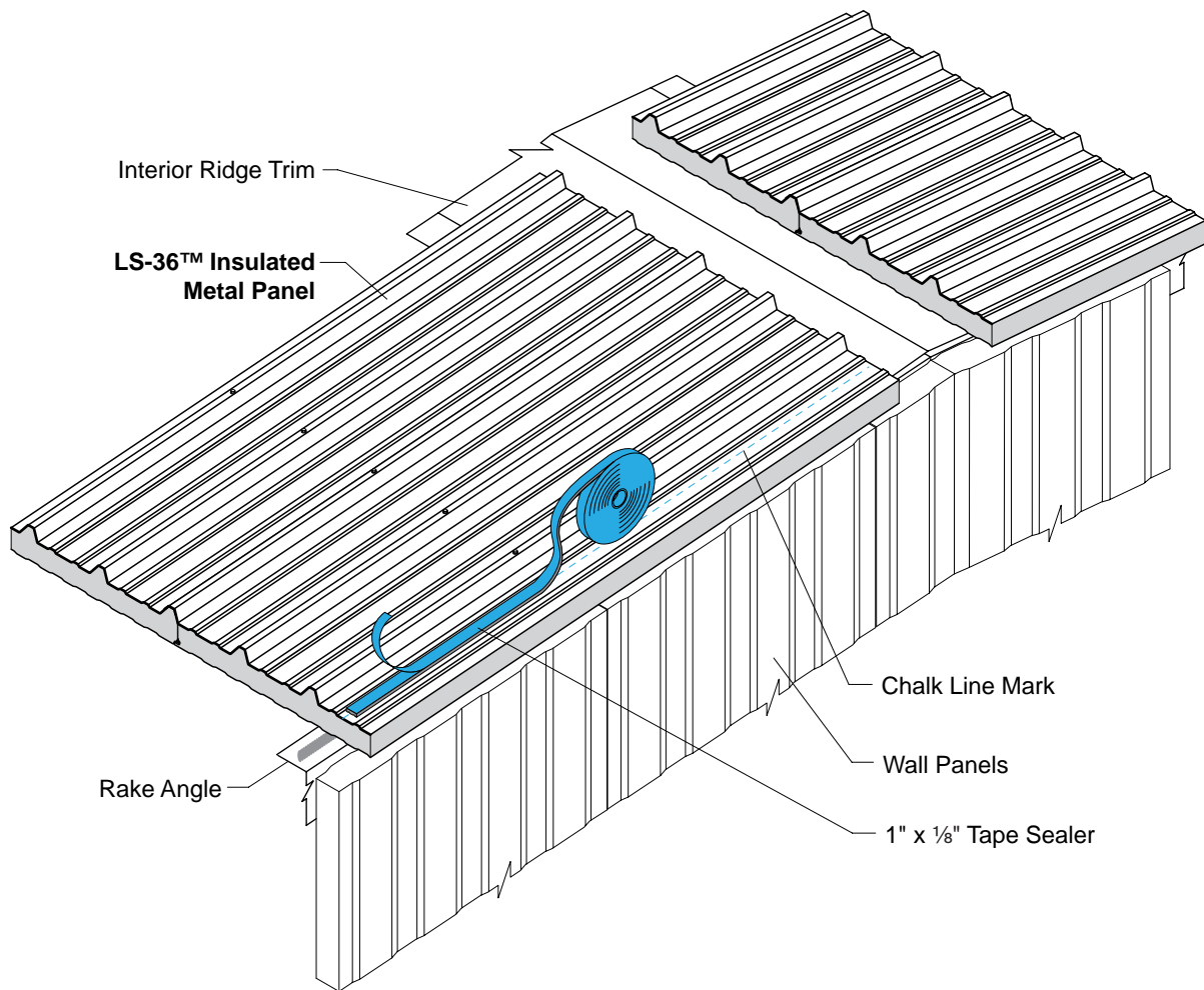
Rake Zee Installation of Tape Sealant
