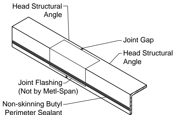
Sealing Structural Joints
