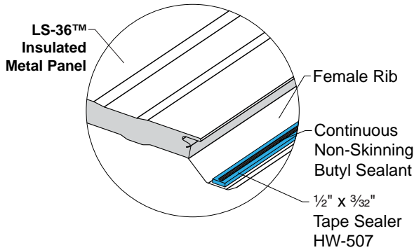
Sidelap Sealant
