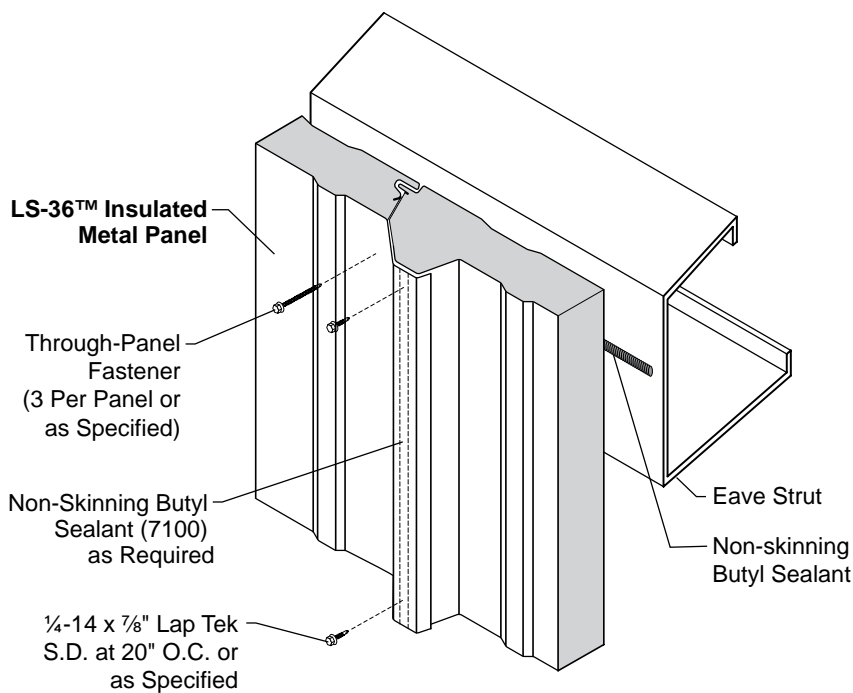
Panel Attachment at Eave/Rake
