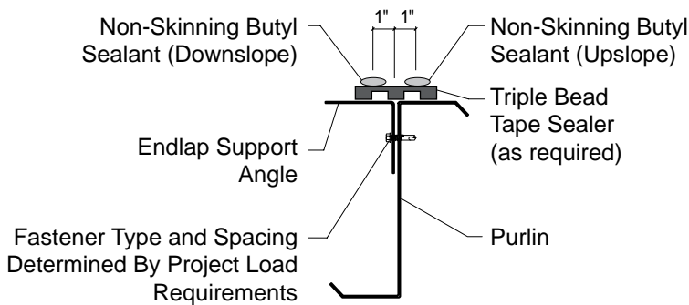
Endlap Vapor Sealant Locations
