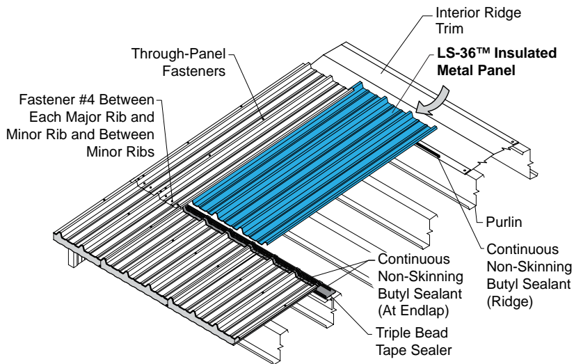
Subsequent Runs Ridge Panel
