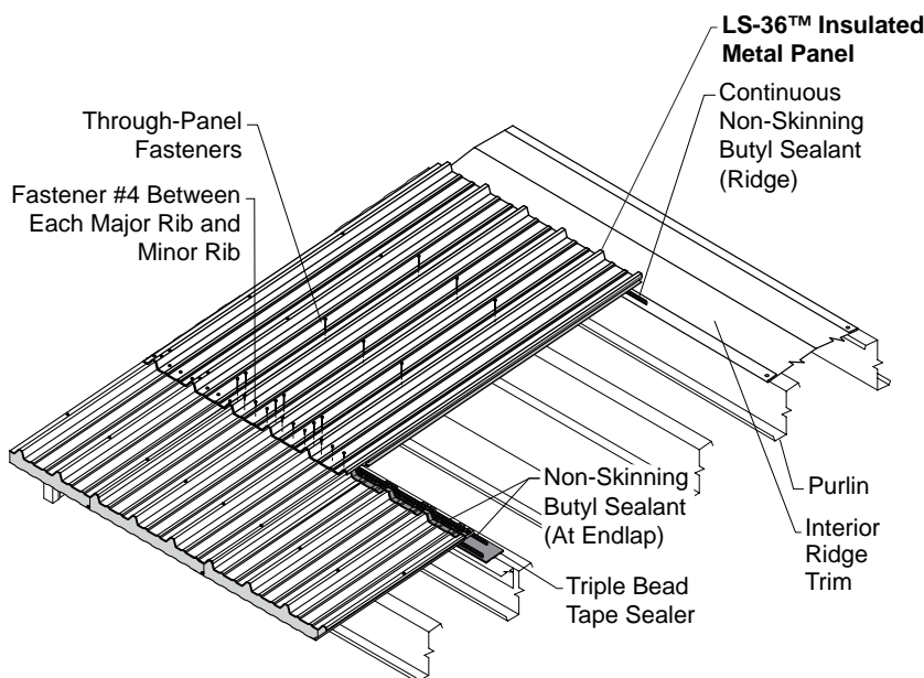
Subsequent Runs Ridge Panel Fastened
