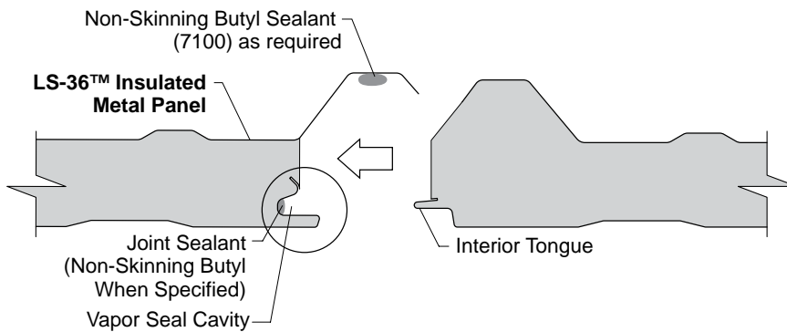
Joint Sealant Application
