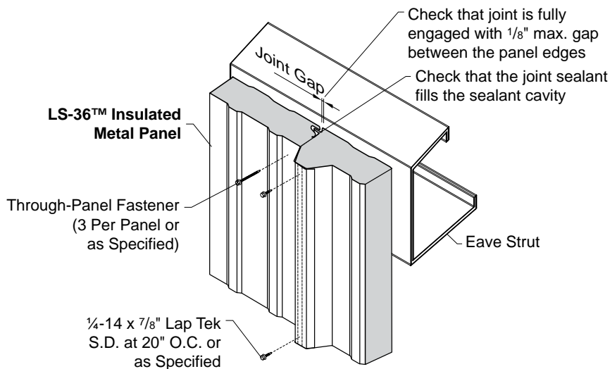
Checking The Panel Joint
