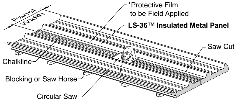
Cutting Panels
