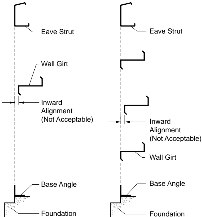
Unacceptable Alignment
