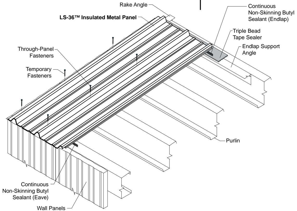
First Panel Fastened
