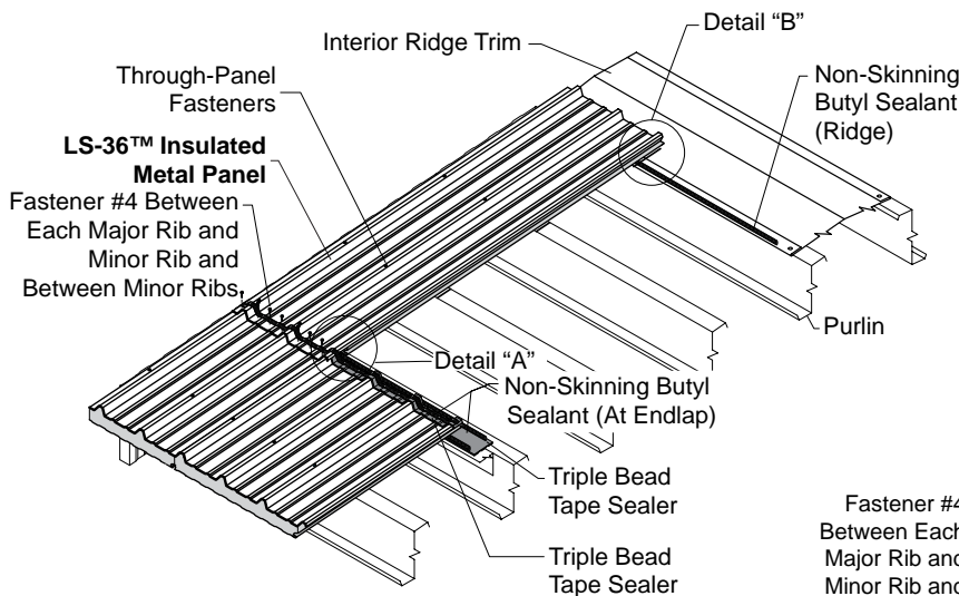
Endlap Panel Attachment
