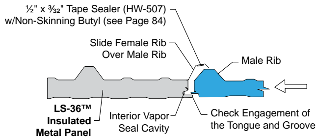
Subsequent Runs Sidelap Engagement
