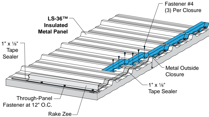
Outside Closure Installation
