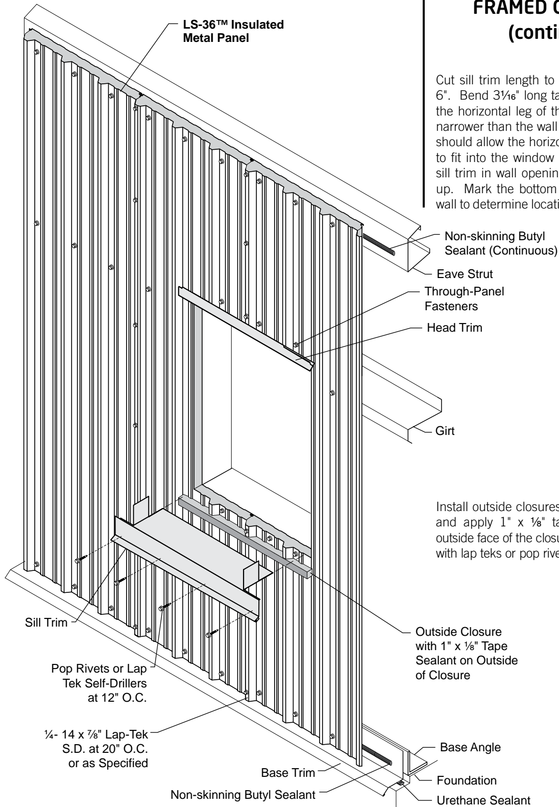
Sill Trim Installation
