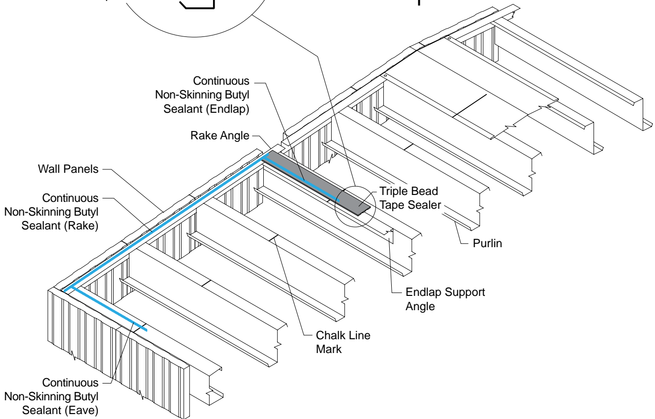
First Panel Vapor Sealant
