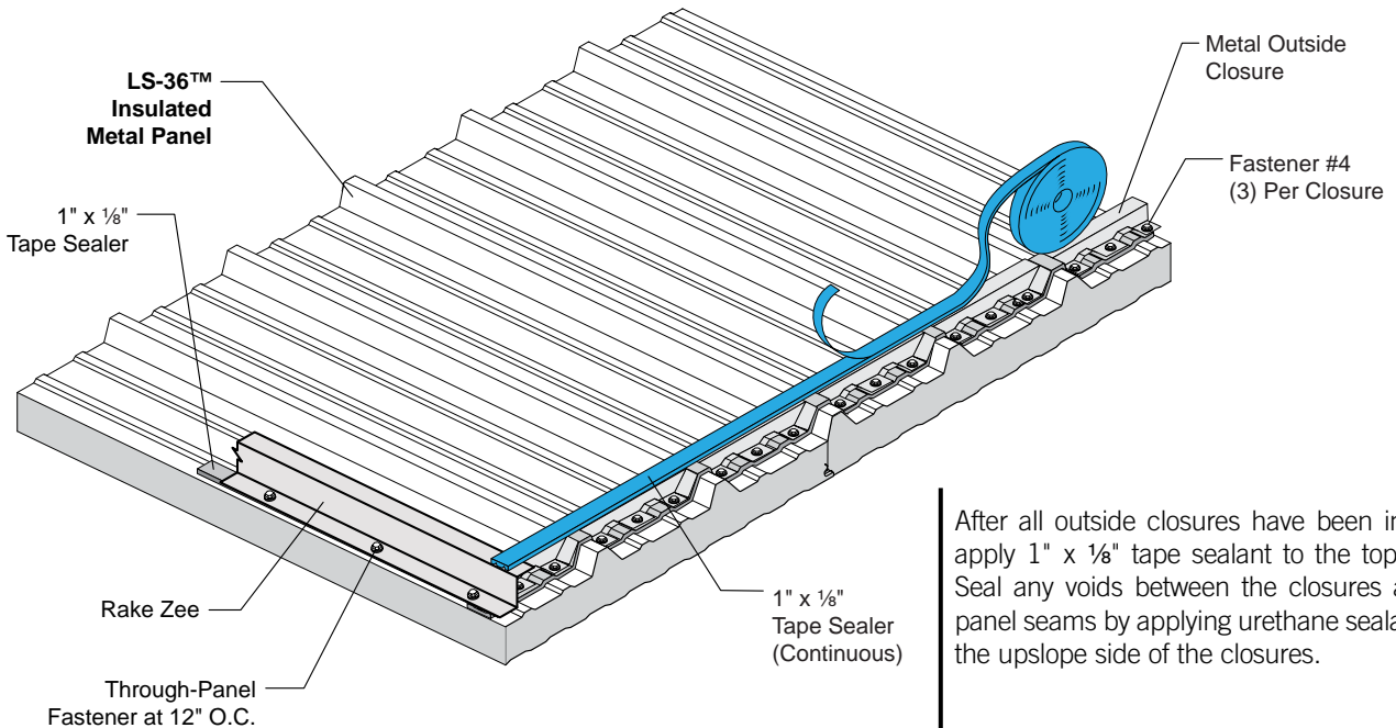
Outside Closure Installation Final
