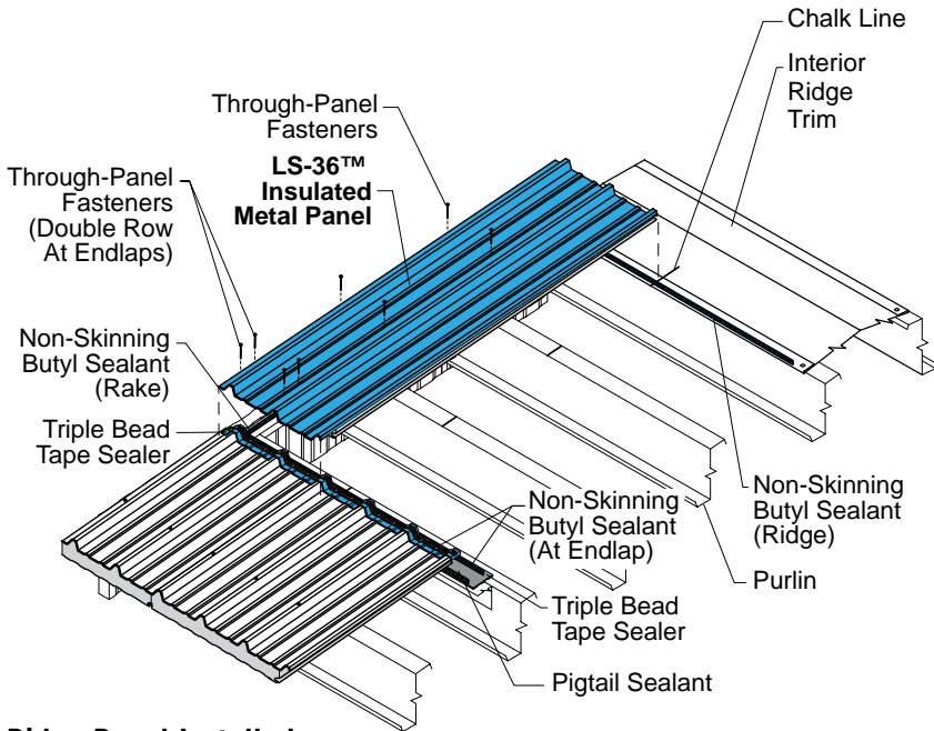
Ridge Panel Installed
