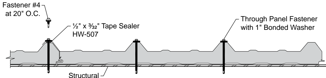
Fastener Patterns at Base, Intermediate and Ridge Structural
