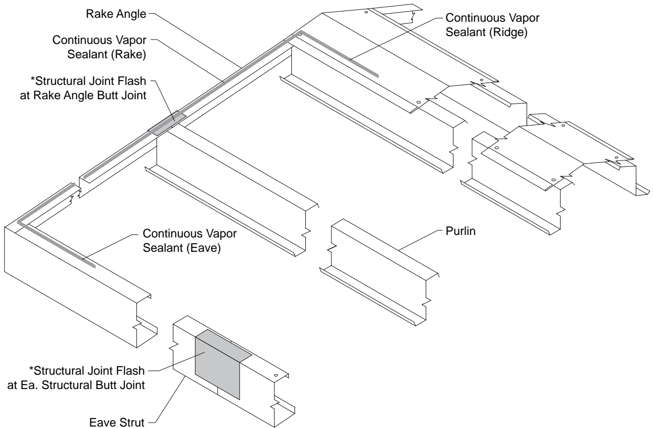
Perimeter Seal
