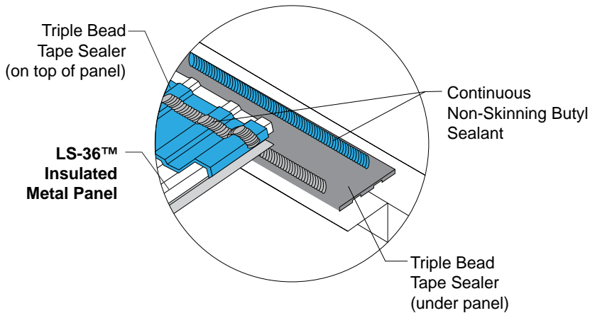
Endlap Installation
