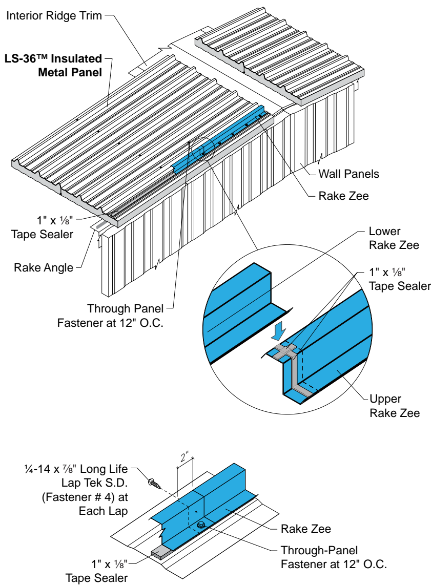
Rake Zee Installation
