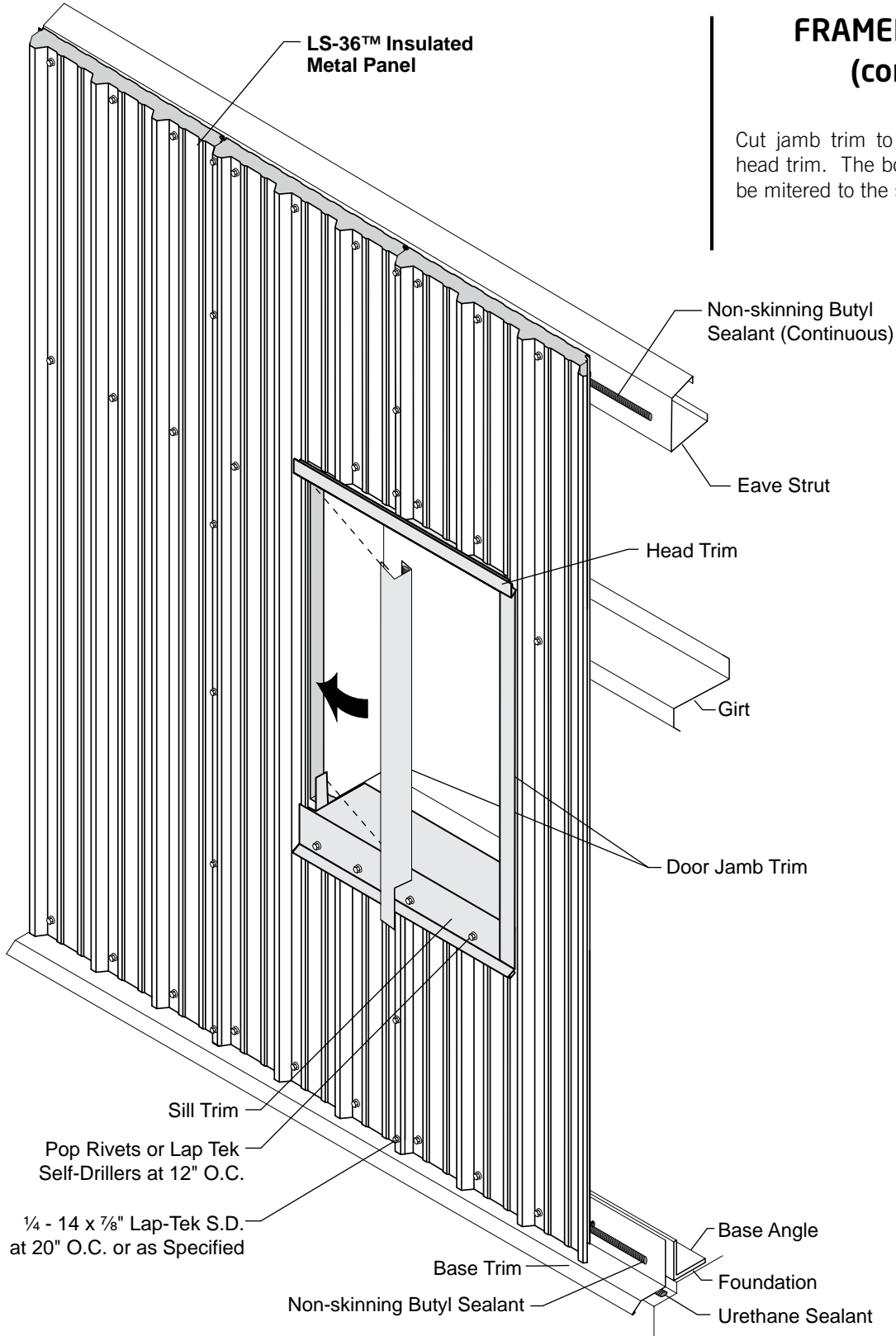
Jamb Trim Installation
