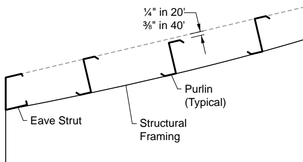
Acceptable Alignment
