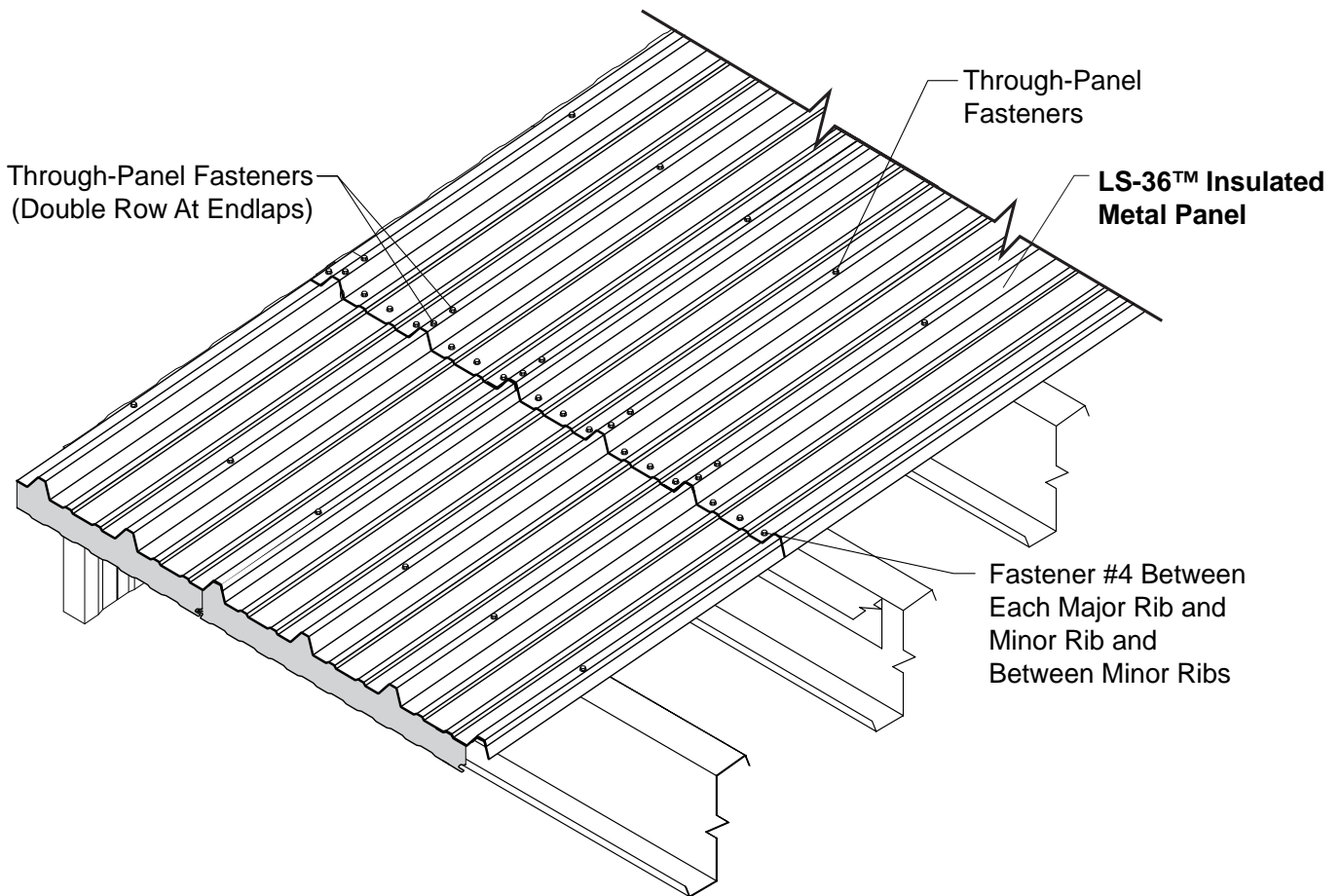
Fastener Patterns at Base, Intermediate and Ridge Structural
