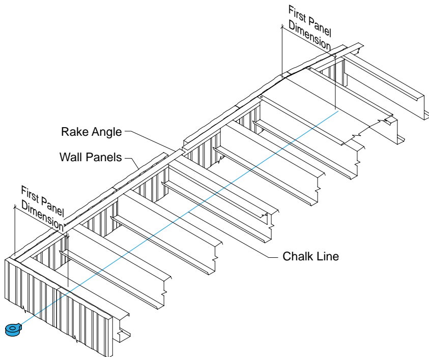
First Panel Chalk Line
