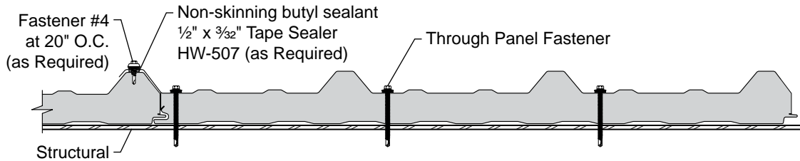
Fastener Pattern at Base, Intermediate and Head Structurals
