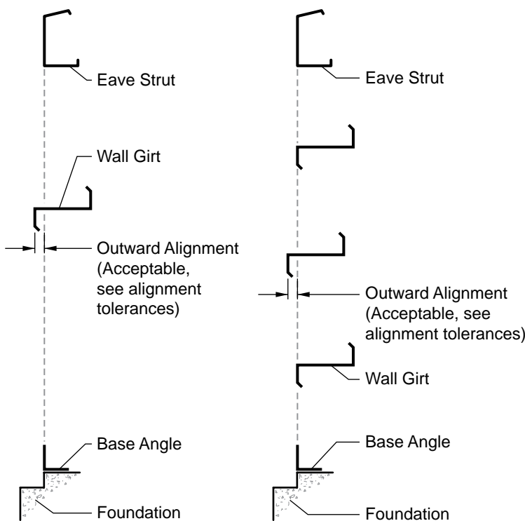
Acceptable Alignment
