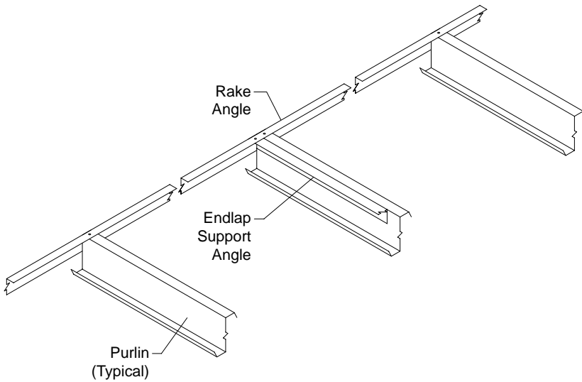
Rake Angle / Endlap Support Angle Installation
