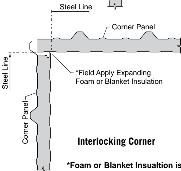
Lapped Corner
