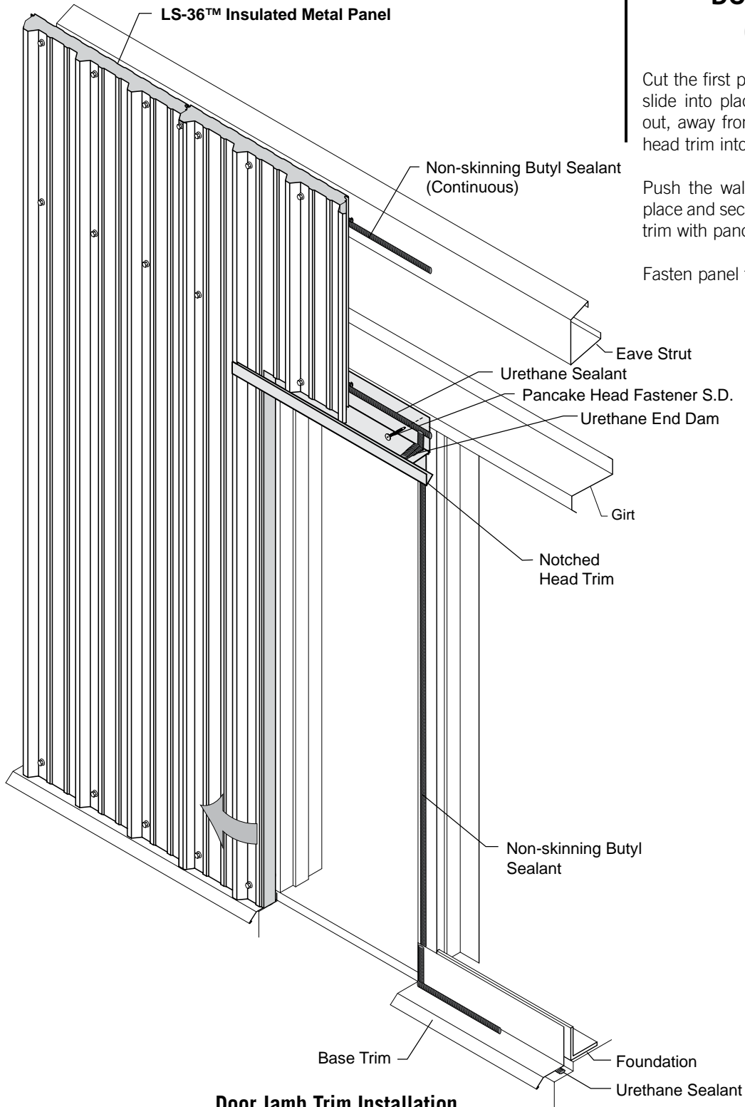
Door Jamb Trim Installation
