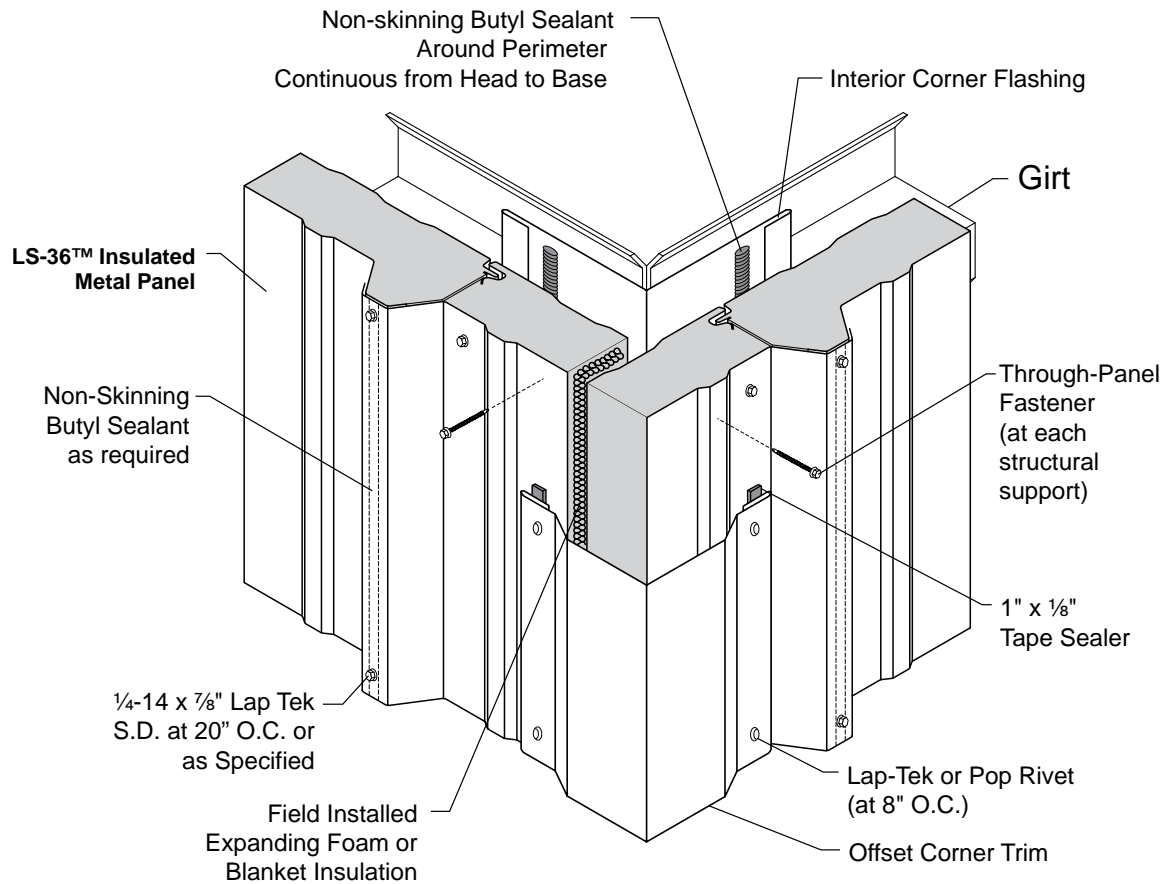
Corner Panel Attachment (Offset Corner Trim)
