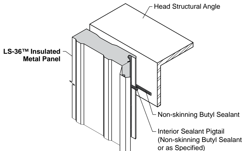
Sealant Pigtail at Head Joint
