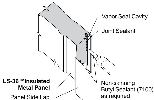
Field Applied Joint Sealant
