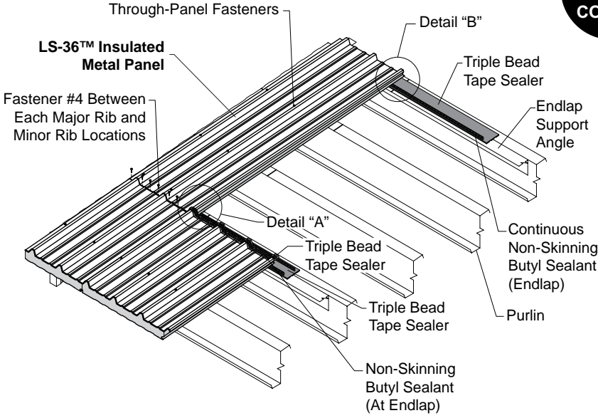
Endlap Panel Attachment
