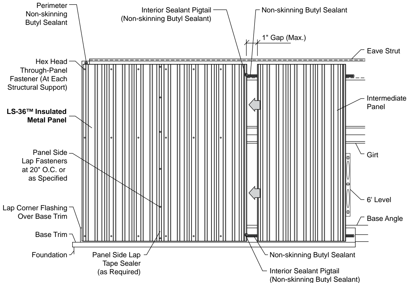
Setting Intermediate Panels
