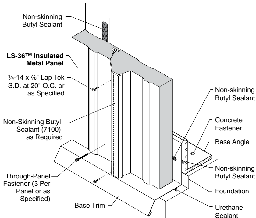
Panel Attachment at Base
