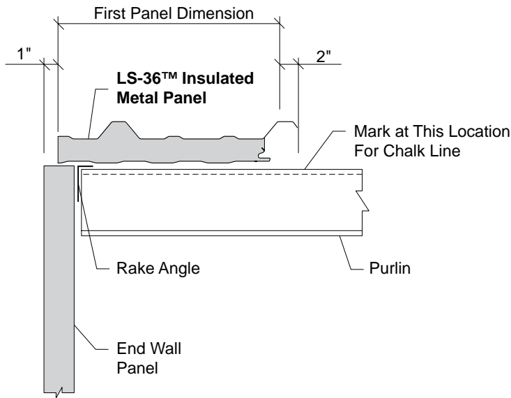
First Panel Section Cut
