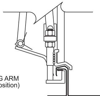
STEP 2 Hand Tool Locked Onto Seam
