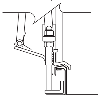
STEP 1 Hand Tool Positioned Over Seam
