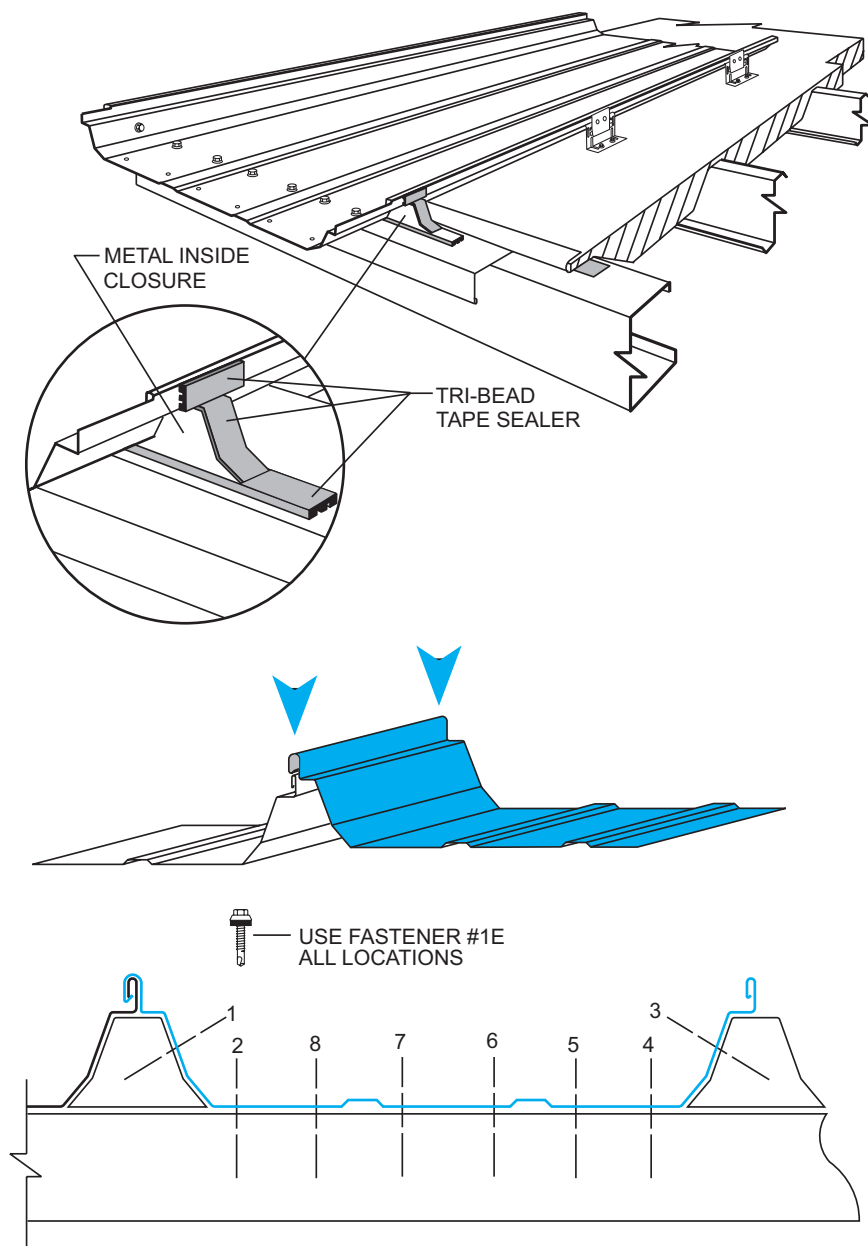
FASTENER SEQUENCE SUBSEQUENT RUNS - EAVE
